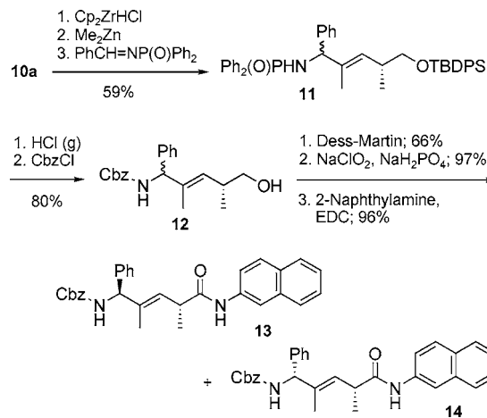
Scheme 2. Synthesis of Methyl-Substituted ( E )-Alkene Dipeptide Isosteres
