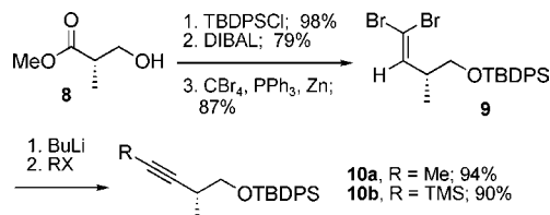
Scheme 1. Synthesis of Methyl- and TMS-Substituted Alkynes
